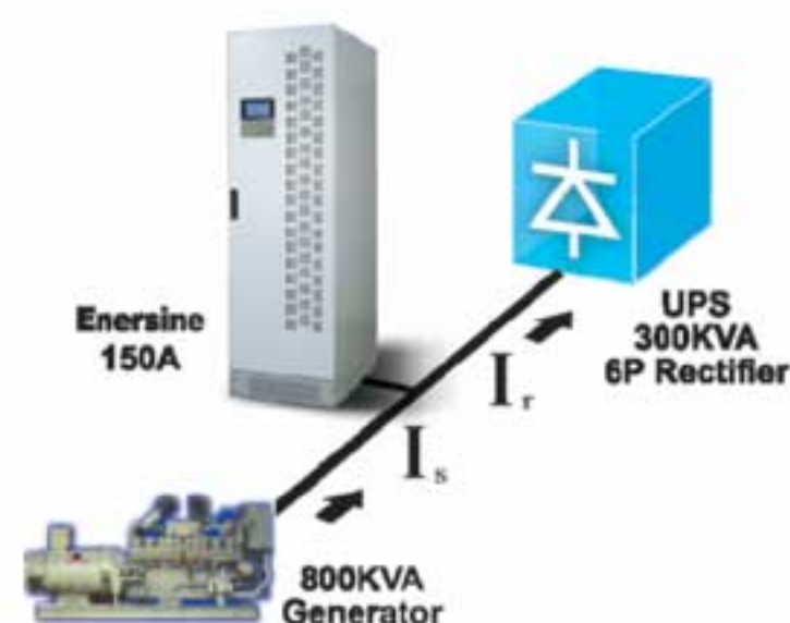
V & Is/Ir while Enersine off THDV=17.4%
