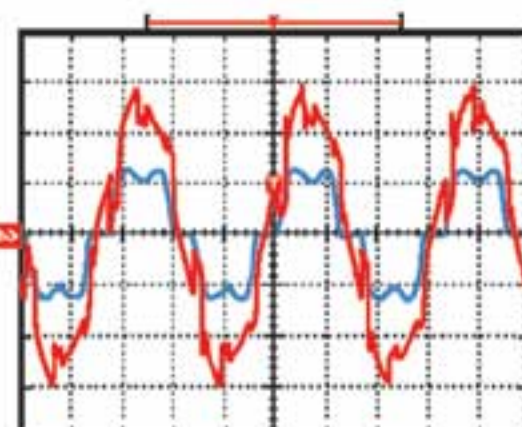
V & Is/Ir while Enersine off THDV=17.4%
