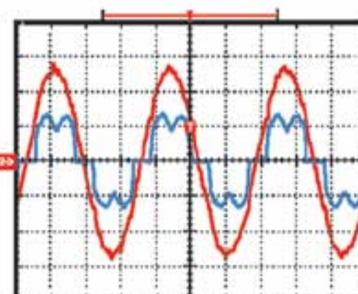
V & Ir while Enersine on THDV=3.1%, THDIr=30.0%
